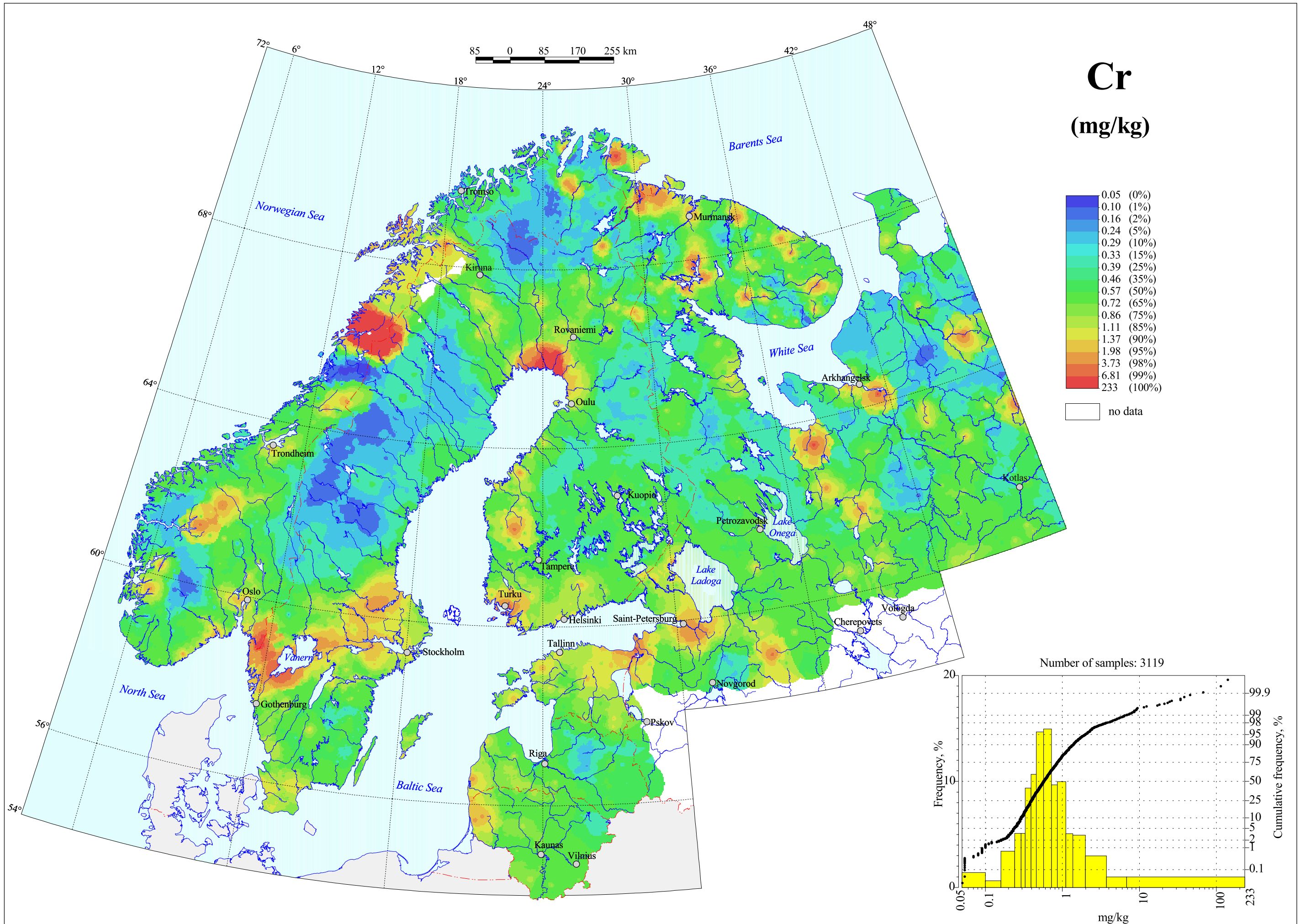
Chromium in Terrestrial Moss, Total Content
